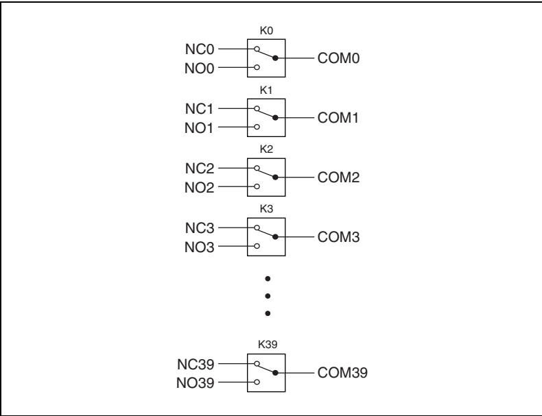
Figure 1. NI PXI-2570 Configuration (Relay Shown in Power-On State)
