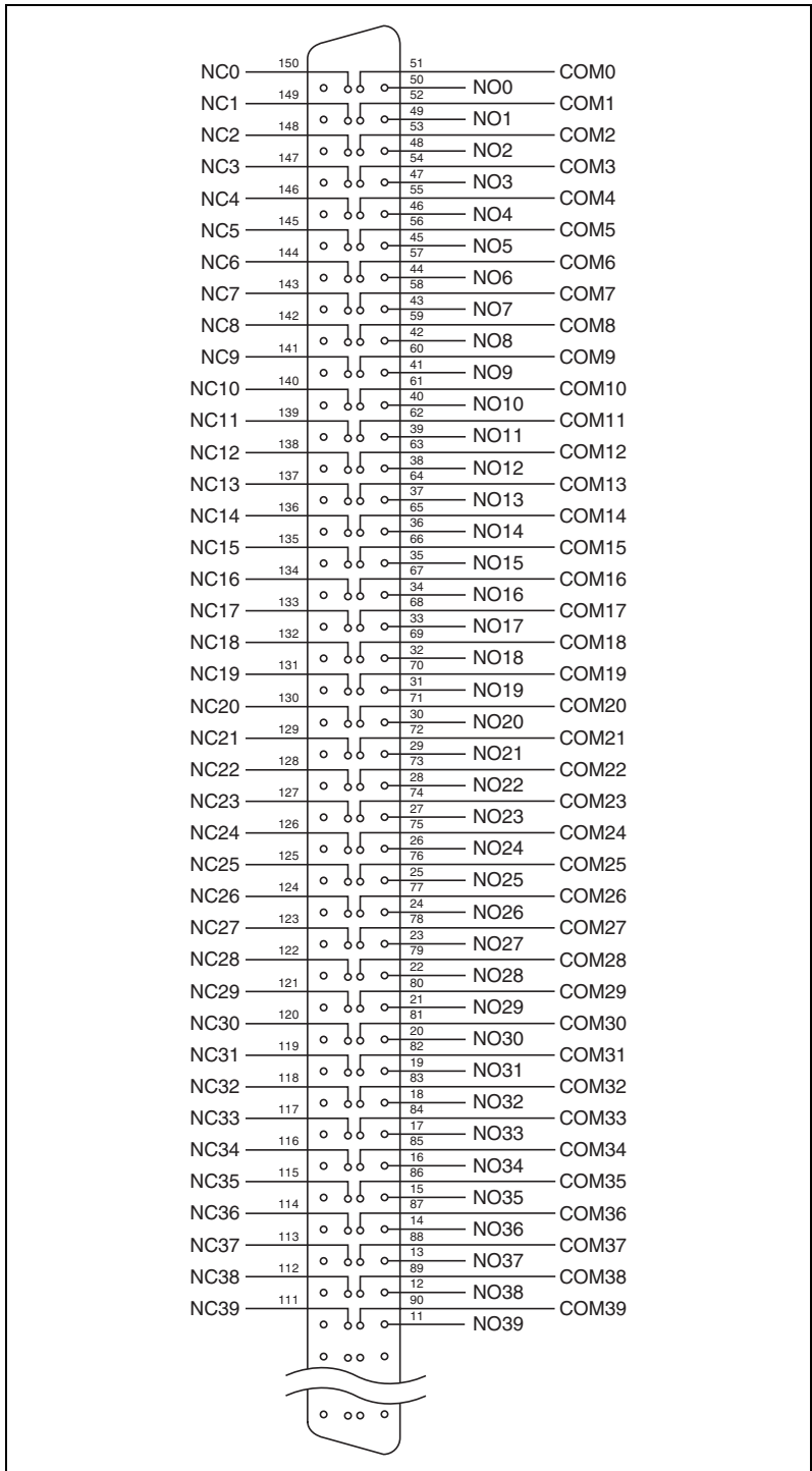
Figure 2. NI PXI-2570 Front Connector Pinout
